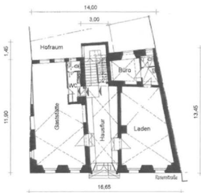
Grundriß Erdgeschoß
